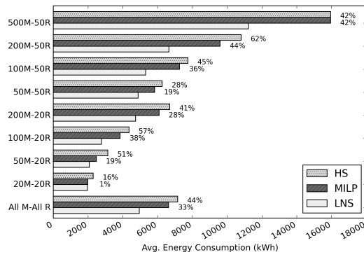
Figure 4: Performance of LNS, MILP and HS.
