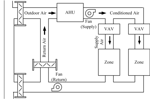
Figure 1: VAV System with Two Zones
