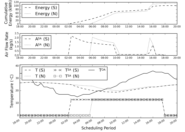
Figure 3: HVAC control with and without standby mode.
