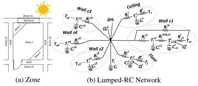
Figure 2: Thermal Model
