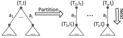
Figure 3: The PARTITION function.
