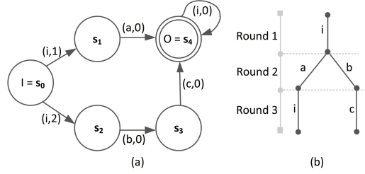
Figure 1: (a) Transition relation \delta in Example 1; (b) Example abstract game trees.
