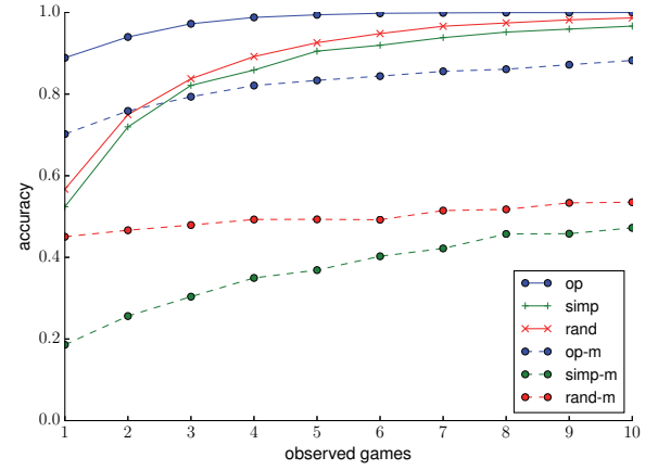
Figure 3: Classification accuracy in tic-tac-toe. Solid lines denote an SNB classifier with PSDDs. Dashed lines denote an NB classifier with Mallows models.
