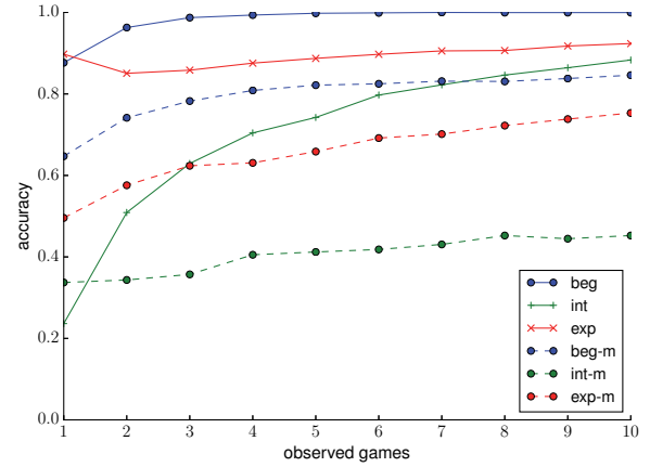
Figure 5: Classification accuracy in 3 \times 3 Hex. Solid lines denote an SNB classifier with PSDDs. Dashed lines denote an NB classifier with Mallows models.
