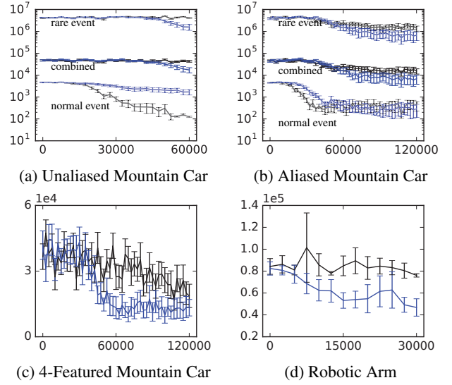
Figure 1: Average per-episode penalty on the orig. MDP (lower is better) for OFFER (blue) and baseline PG (black).
