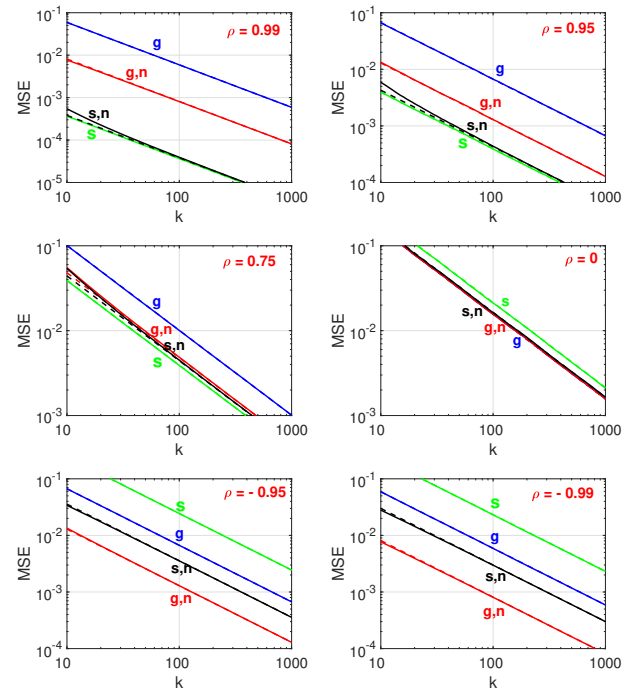
Figure 3: Empirical MSEs (solid curves) for four proposed estimators, together with theoretical (asymptotic) variances (dashed curves), for 6 \rho values. For \hat{\rho}_g and \hat{\rho}_s , the solid and dashed curves overlap, confirming that they are unbiased and the variance formulas are correct. For \hat{\rho}_{g,n} and \hat{\rho}_{s,n} , the solid and dashed curves overlap when k is not too small.
