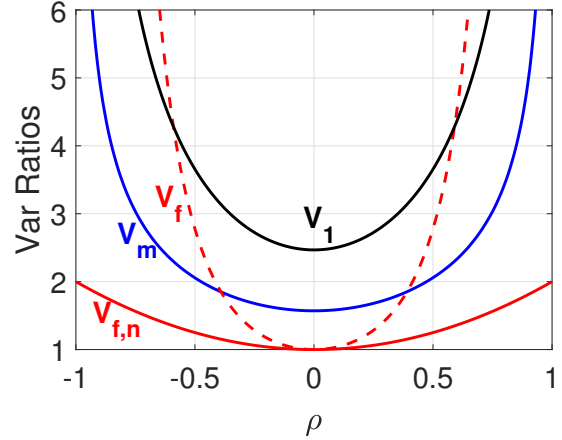
Figure 1: Ratios (lower the better) of variance factors: \frac{V_1}{V_{f,m}} , \frac{V_f}{V_{f,m}} , \frac{V_{f,n}}{V_{f,m}} . They are always larger than 1, as V_{f,m} is the theoretically smallest variance factor. Note that V_m is the variance factor for the MLE of sign-full random projections.
