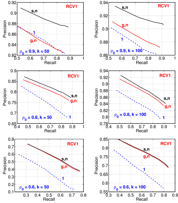
Figure 6: RCV1 : precision-recall curves for selected \rho_0 and k values, and for three estimators: \hat{\rho}_{s,n} , \hat{\rho}_{g,n} , \hat{\rho}_1 .
