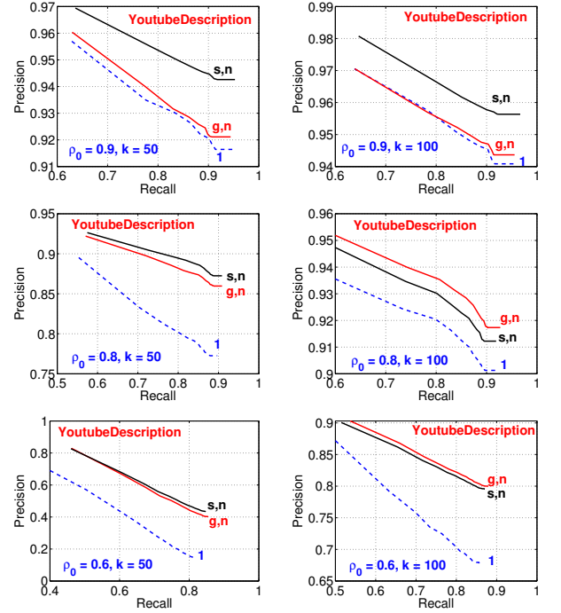
Figure 9: YoutubeDescription : precision-recall curves for selected \rho_0 and k values, and three estimators: \hat{\rho}_{s,n} , \hat{\rho}_{g,n} , \hat{\rho}_1 .
