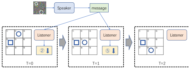
Figure 6: Object Placement task. Speaker observes the target state (image) and describes it to Listener. Listener observes the grid world containing the two objects and receives the message from Speaker. Then it moves the objects to place them to form the correct positional relationship as depicted in the target state.
