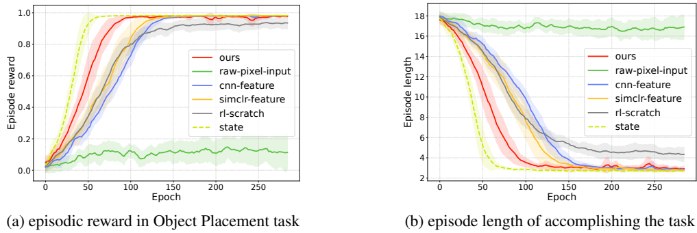
Figure 7: Performance of new Listener trained with different inputs of the target state in the Object Placement task. All experiments are run for 5 seeds, and the shaded part of the curves is one standard error.
