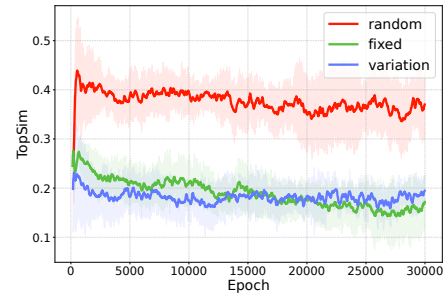
Figure 5: TopSim of agents trained with different datasets.
