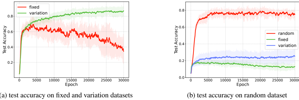
Figure 2: Test accuracy of agents. (a) Agents trained with the fixed dataset or variation dataset are tested using the corresponding test set. (b) Agents trained with three kinds of datasets are tested with the test set of the random dataset.
