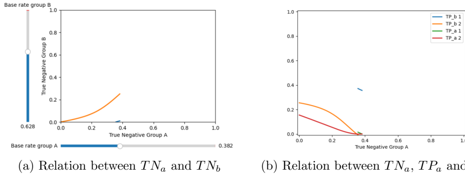
Figure 4: Relation between the free variable TN_a and the variables TN_b, TP_a, TP_b for (PP, FORP, OaE), showing multiple values are possible for TP_b and TP_a given TN_a .
