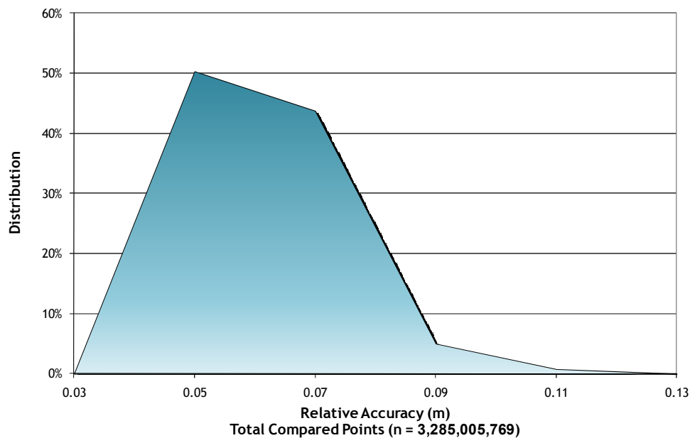
Figure 4.1. Distribution of relative accuracies, non slope-adjusted.
