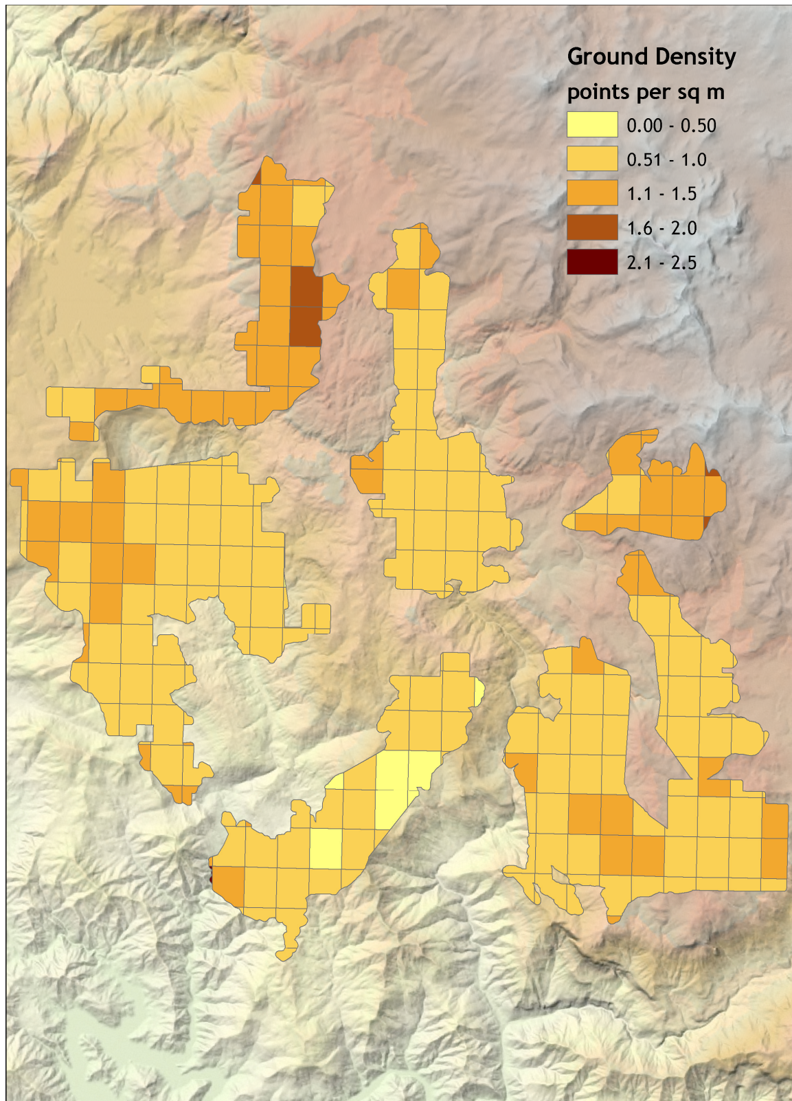
Figure 4.10. Ground-classified laser point data density for the Dinkey Creek study area (UTM11), displayed over a 30m DEM.
