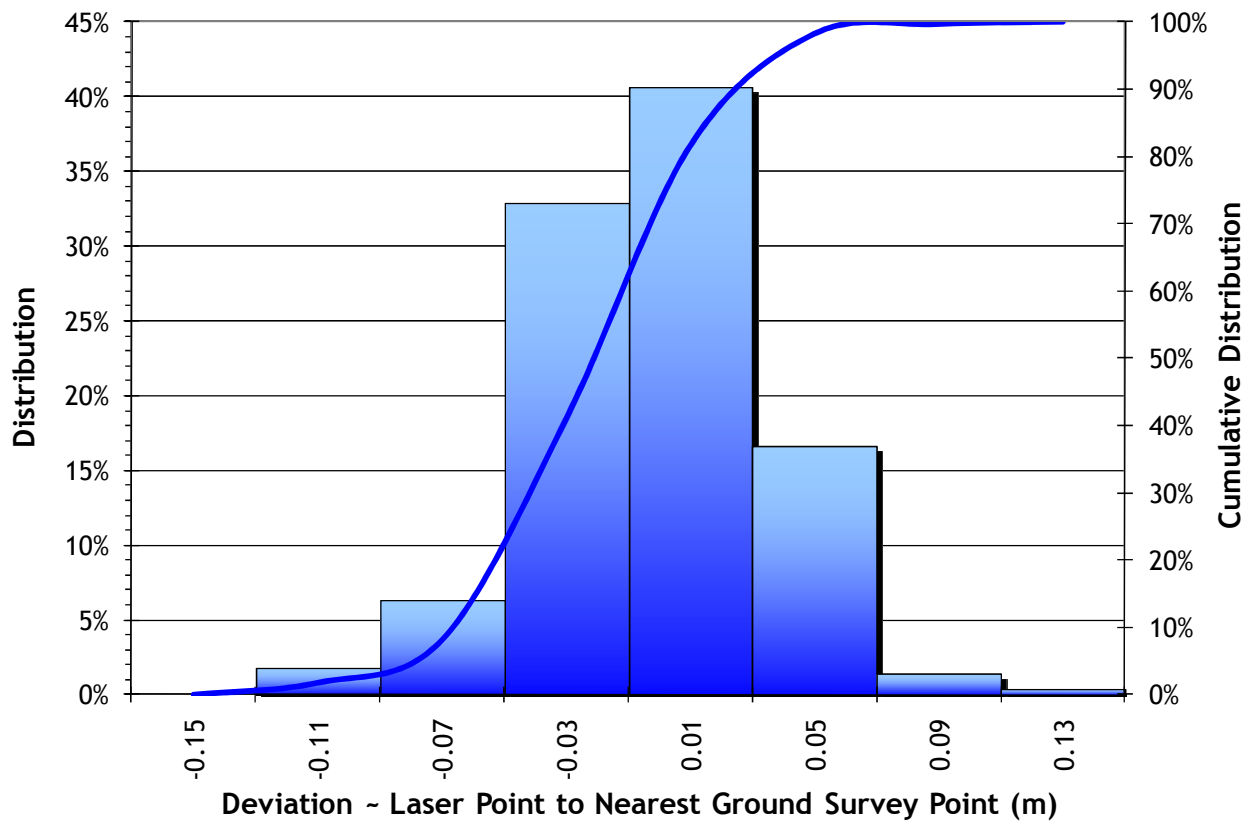
Figure 4.3. Histogram statistics, calculated from 283 hard surface calibration points.
