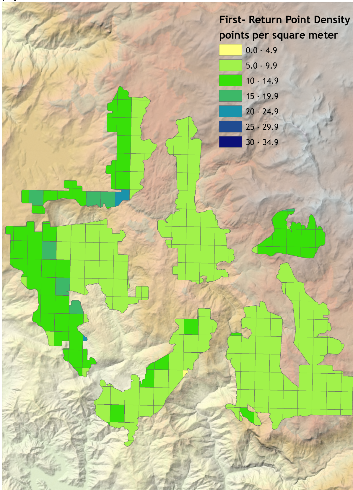
Figure 4.7. First return laser point data density for the Dinkey Creek, Tea Kettle study area (UTM11), displayed over a 30m DEM.
