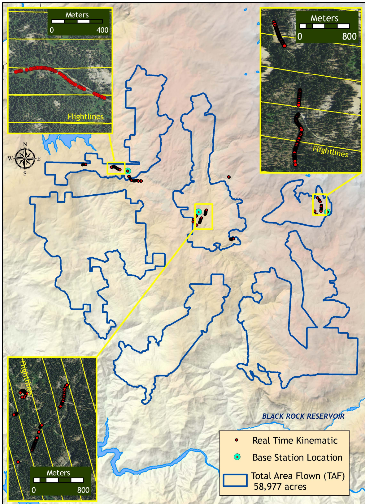
Figure 2.3. Sample selection of RTK points in the Dinkey Creek/ Teak Kettle study area, displayed over 30 meter DEM.
