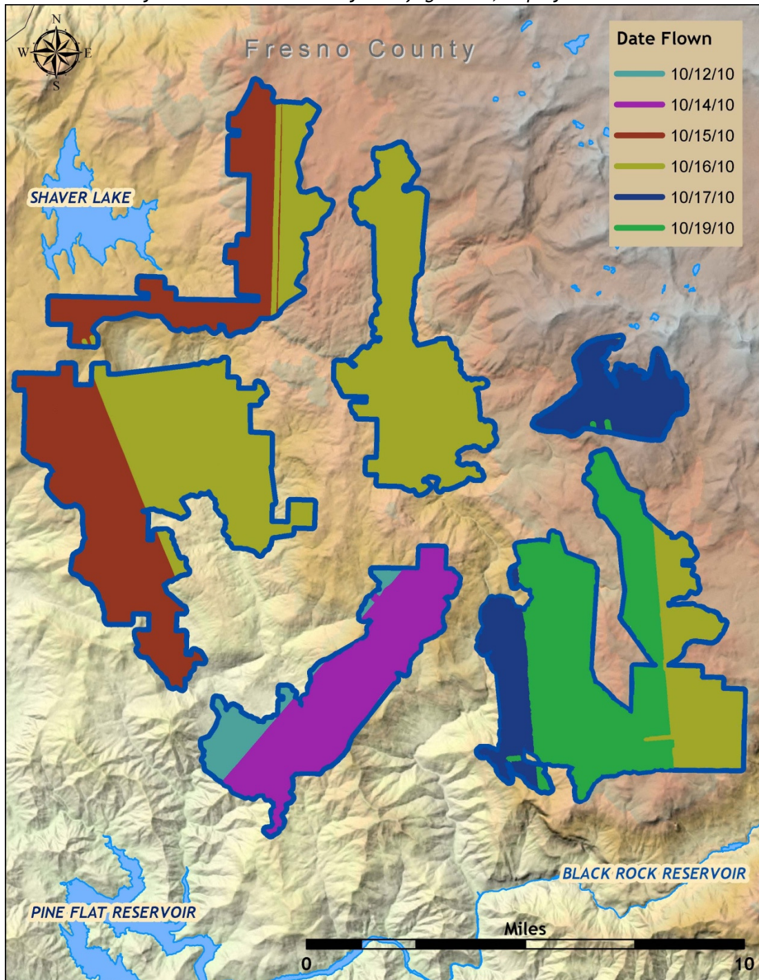
Figure 2.1. The Dinkey Creek/ Tea Kettle study area flightlines, displayed over 30 meter DEM.
