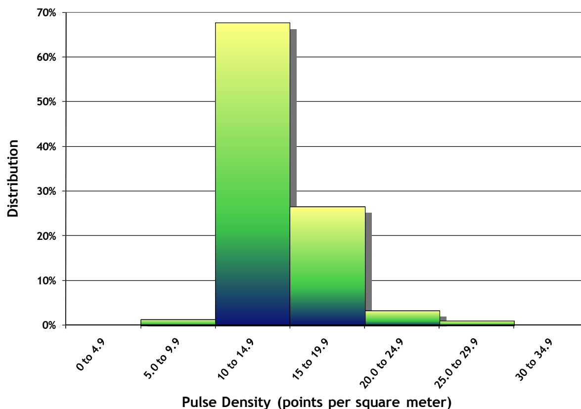
Figure 4.6. Histogram of first return laser point density for the Dinkey Creek and Tea Kettle study area.
