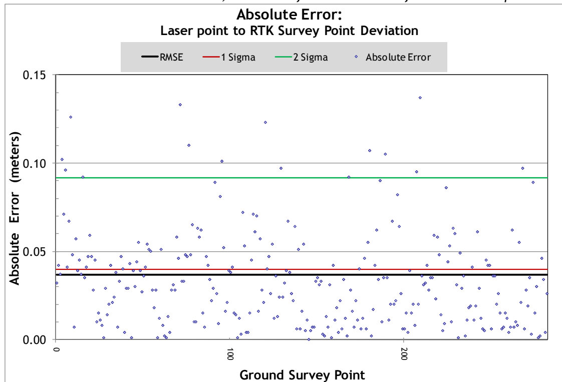
Figure 4.4. Absolute deviation statistics, calculated from 283 hard surface calibration points.
