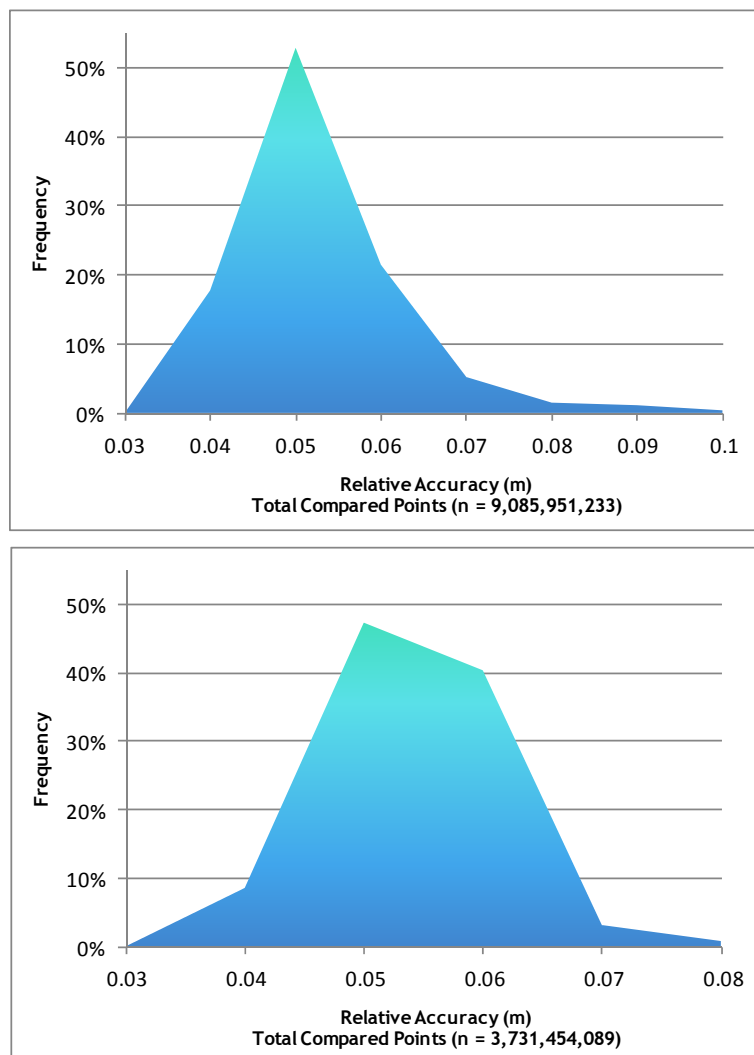
Figure 6. Distribution of relative accuracies for the Kern Plateau North (top) and South (bottom) AOIs per flight line, non slope-adjusted.
