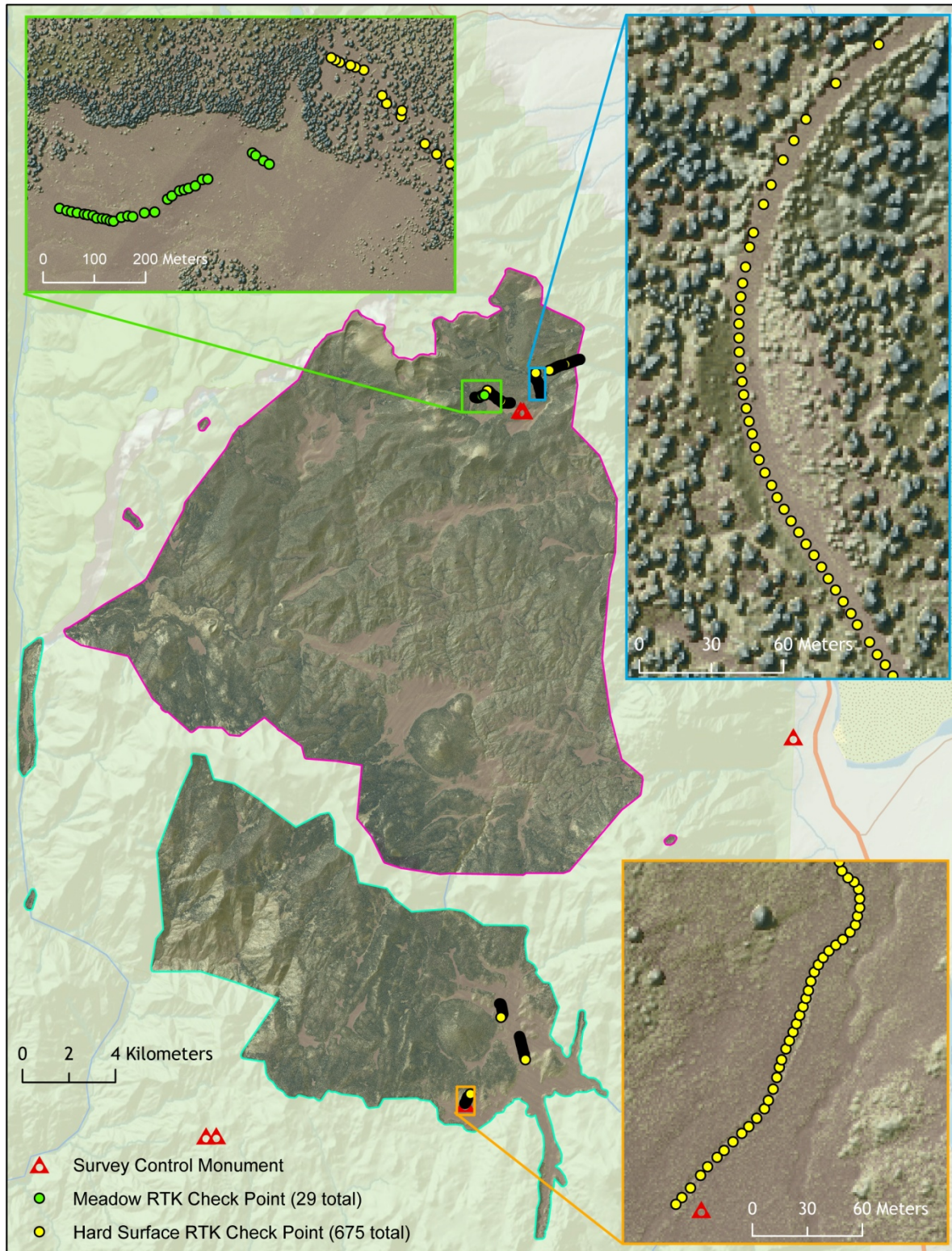
Figure 2. RTK and survey control monument locations used for the Kern Plateau survey area.
