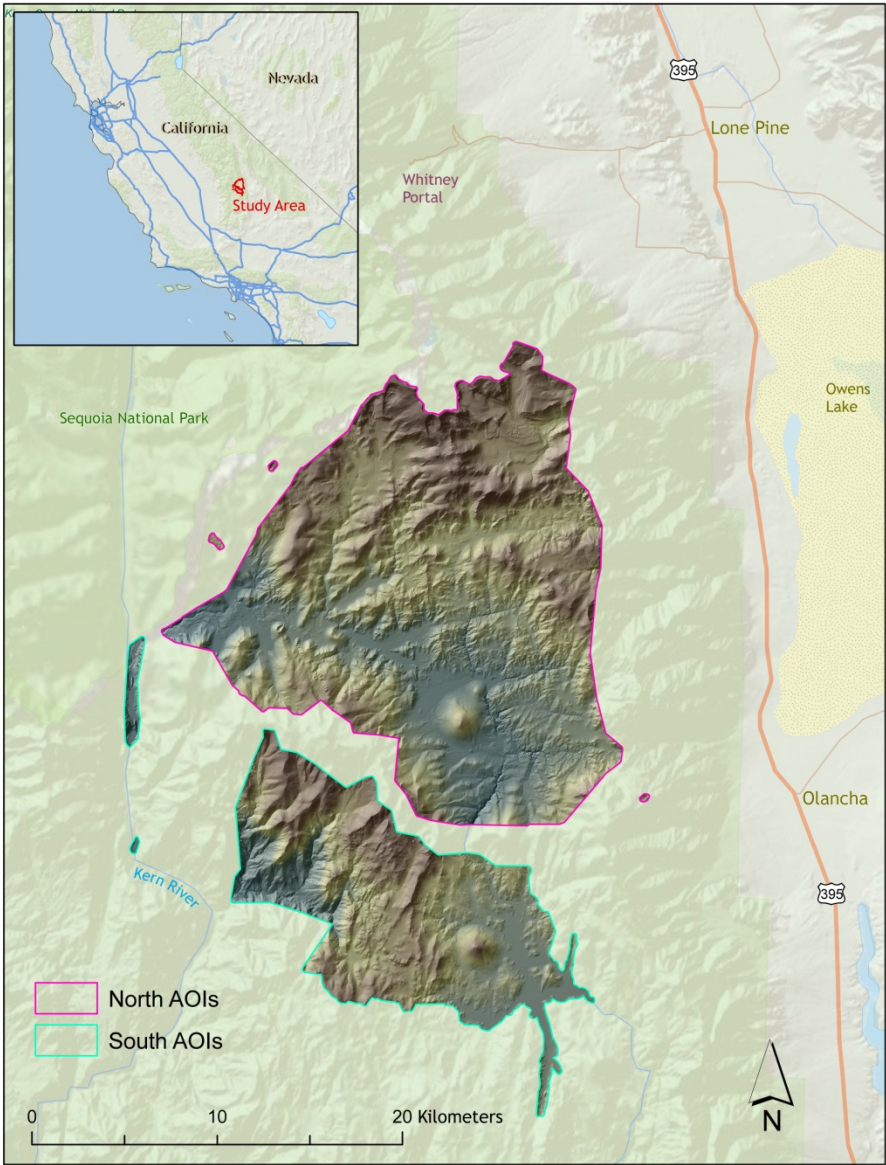
Figure 1. Kern Plateau survey area map.
