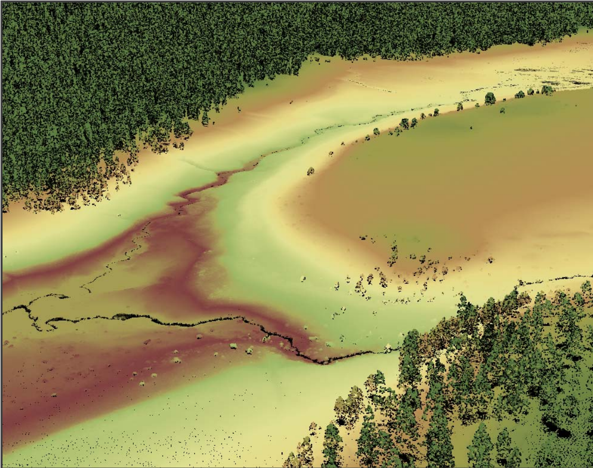
Figure 11. View looking over a portion of Last Chance meadow in the Kern Plateau survey area. Image created from a 3D LiDAR point cloud colored by elevation and intensity.
