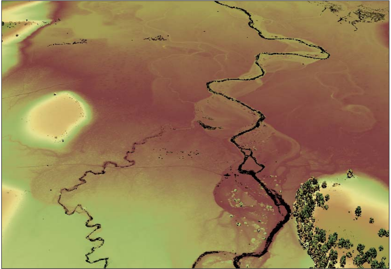
Figure 12. View over a large meadow in the Kern Plateau survey area showing river braiding patterns. Image created from a 3D LiDAR point cloud colored by elevation and intensity.
