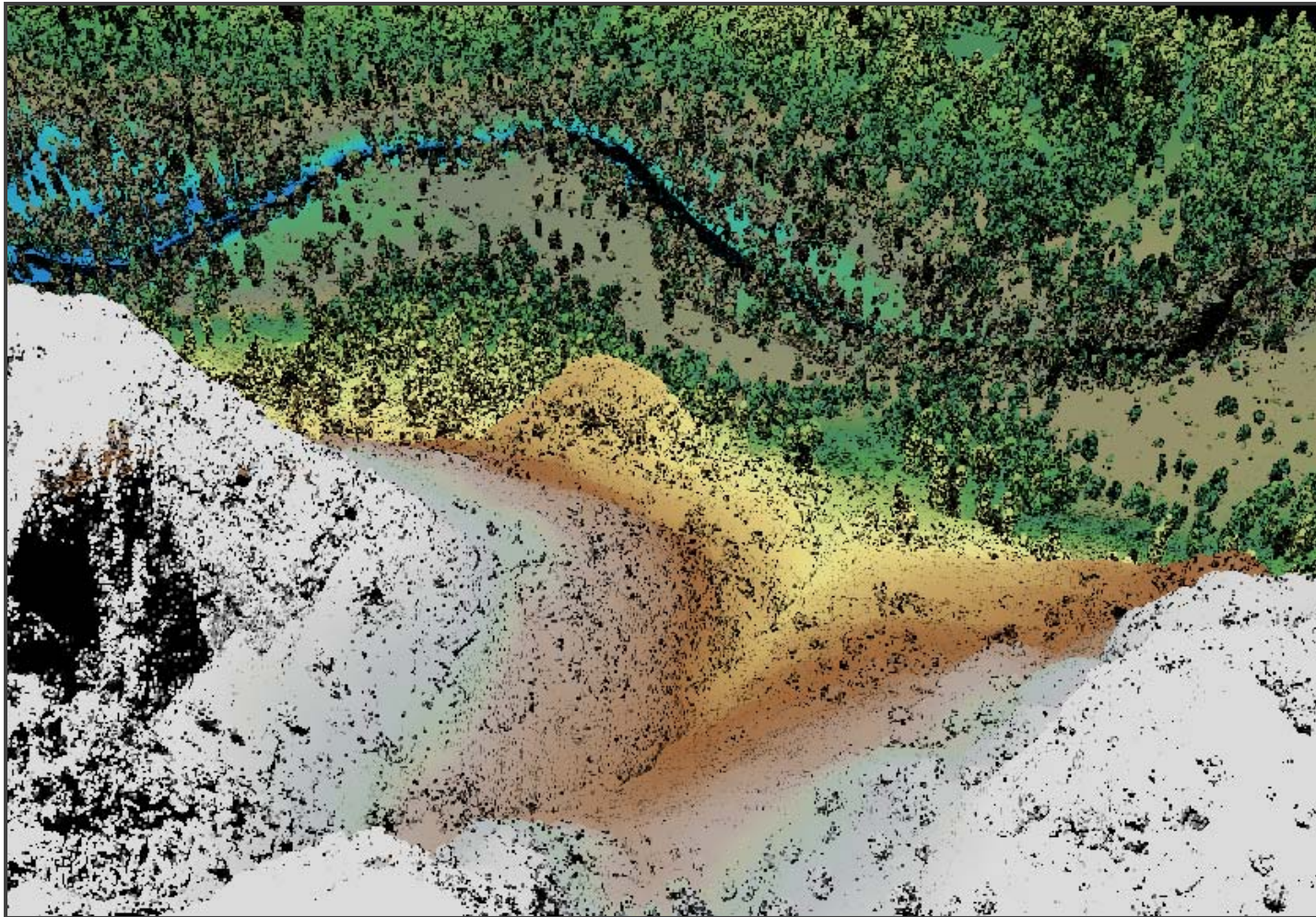
Figure 13. View looking down a steep cliff face to the river below. Image created from a 3D LiDAR point cloud colored by elevation and intensity.
