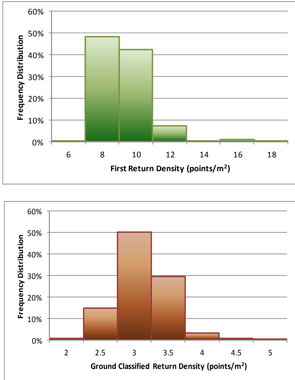
Figure 3. Density distribution for first return (top) and ground classified (bottom) laser points.
