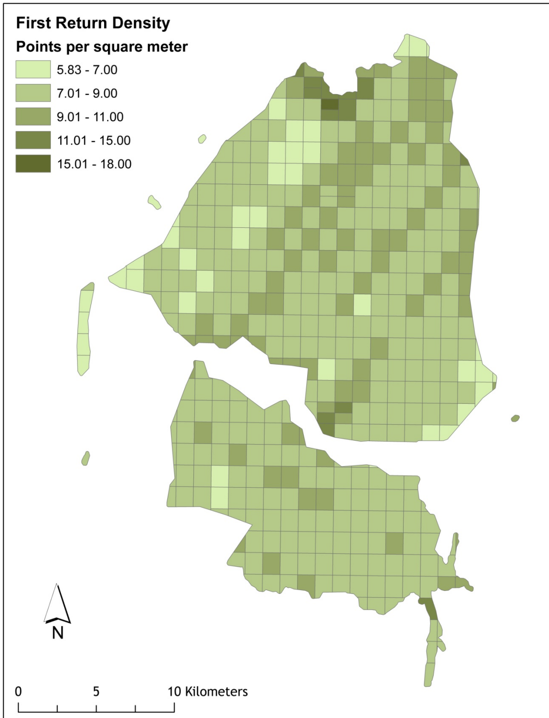
Figure 4. First Return laser point data density per tile.
