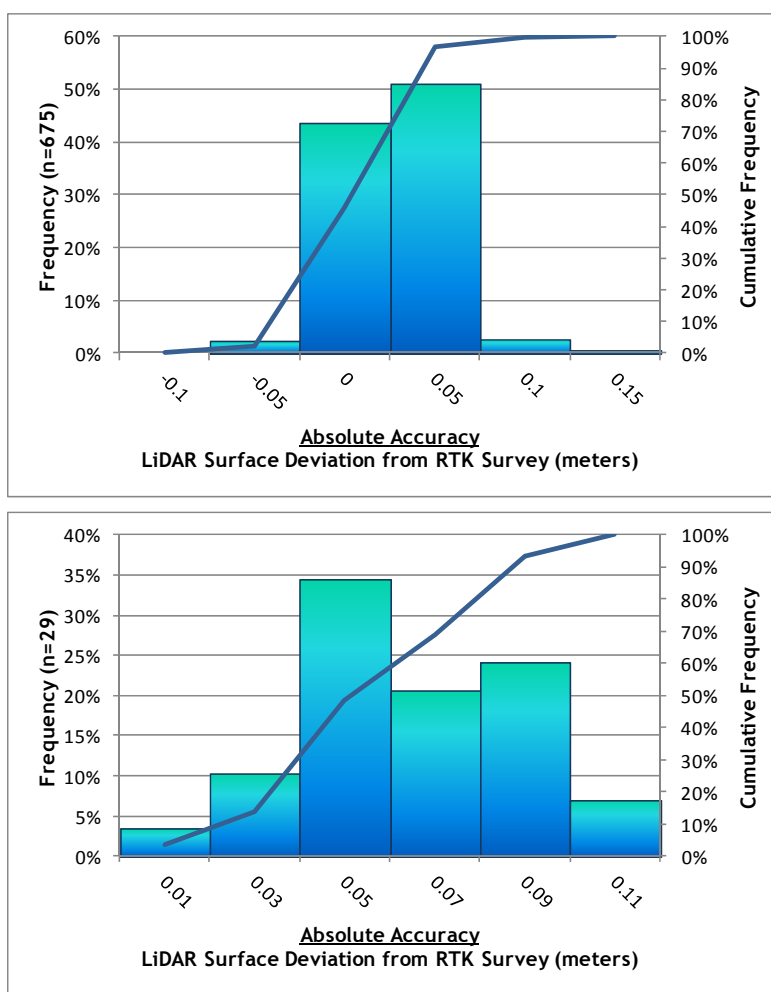
Figure 7. Absolute Accuracy - Histogram Statistics for hard surface points (top) and meadow points (bottom).
