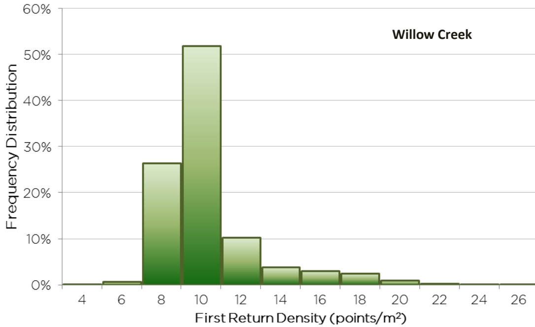
Frequency distribution of first return densities (native densities) of the 1m gridded study area for the Willow Creek AOI
