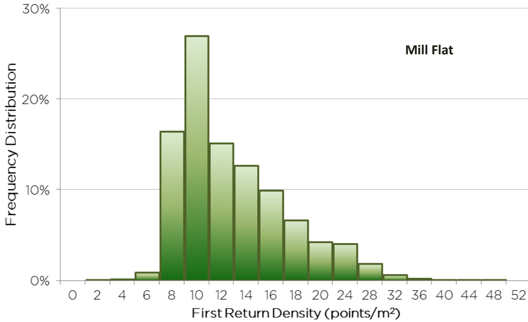
Frequency distribution of first return densities (native densities) of the 1m gridded study area for the Mill Flat AOI
