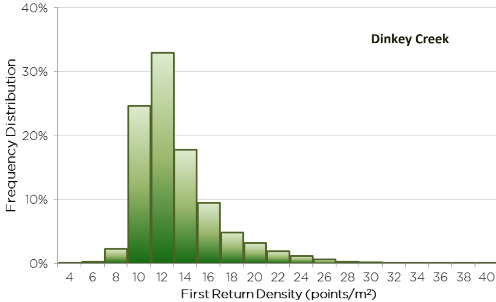
Frequency distribution of first return densities (native densities) of the 1m gridded study area for the Dinkey Creek AOI
