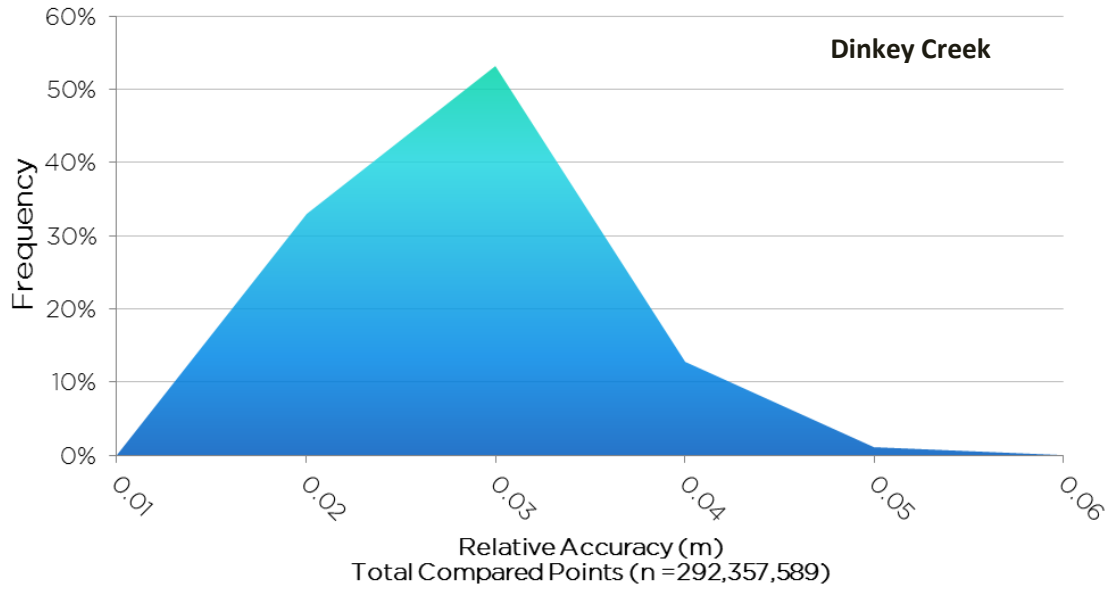
Frequency plot for relative accuracy between flight lines for the Dinkey Creek AOI
