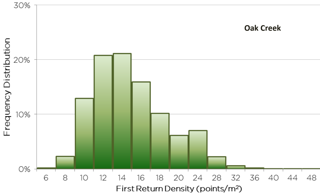
Frequency distribution of first return densities (native densities) of the 1m gridded study area for the Oak Creek AOI
