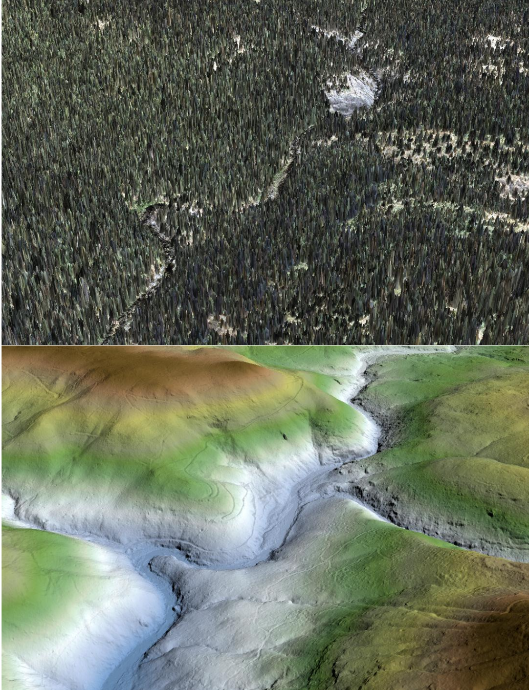
Figure 9: View looking northwest up Dinkey Creek near the confluence of Bear Creek in the Sierra National Forest. Top image created from LiDAR points colored by 2010 NAIP imagery. Bottom image created from ground-classified LiDAR points colored by elevation which illustrates topographic detail normally obscured by vegetation.
