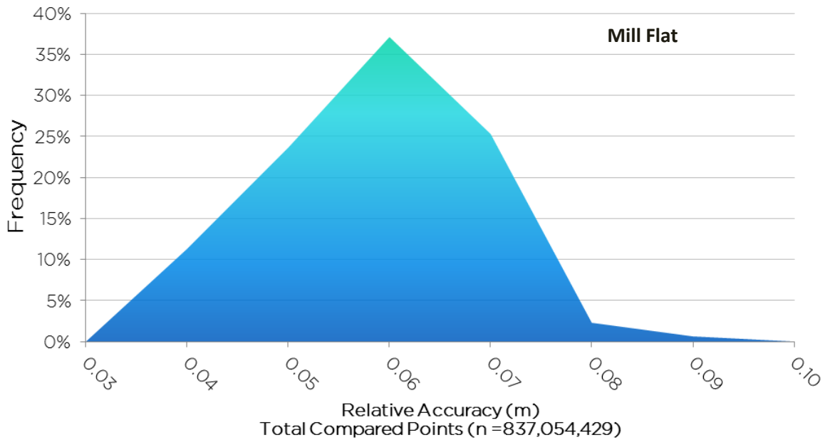
Frequency plot for relative accuracy between flight lines for the Mill Flat AOI
