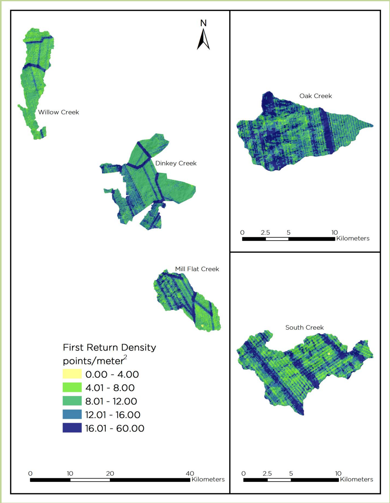
Figure 5: Native density maps for the Central Sierra AOs
