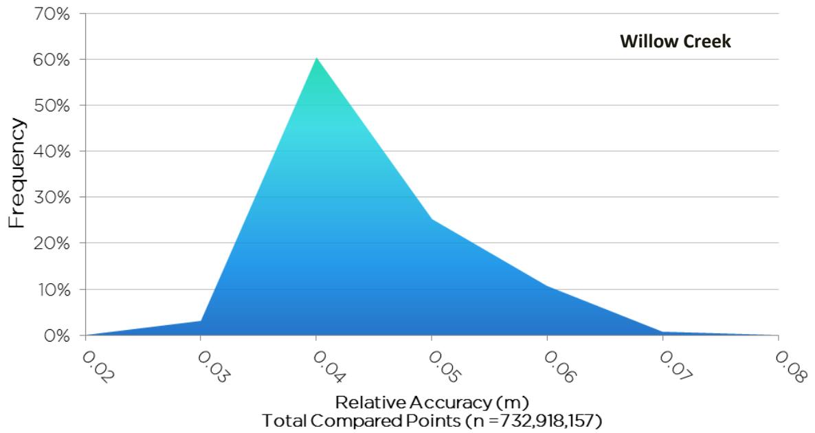
Frequency plot for relative accuracy between flight lines for the Willow Creek AOI
