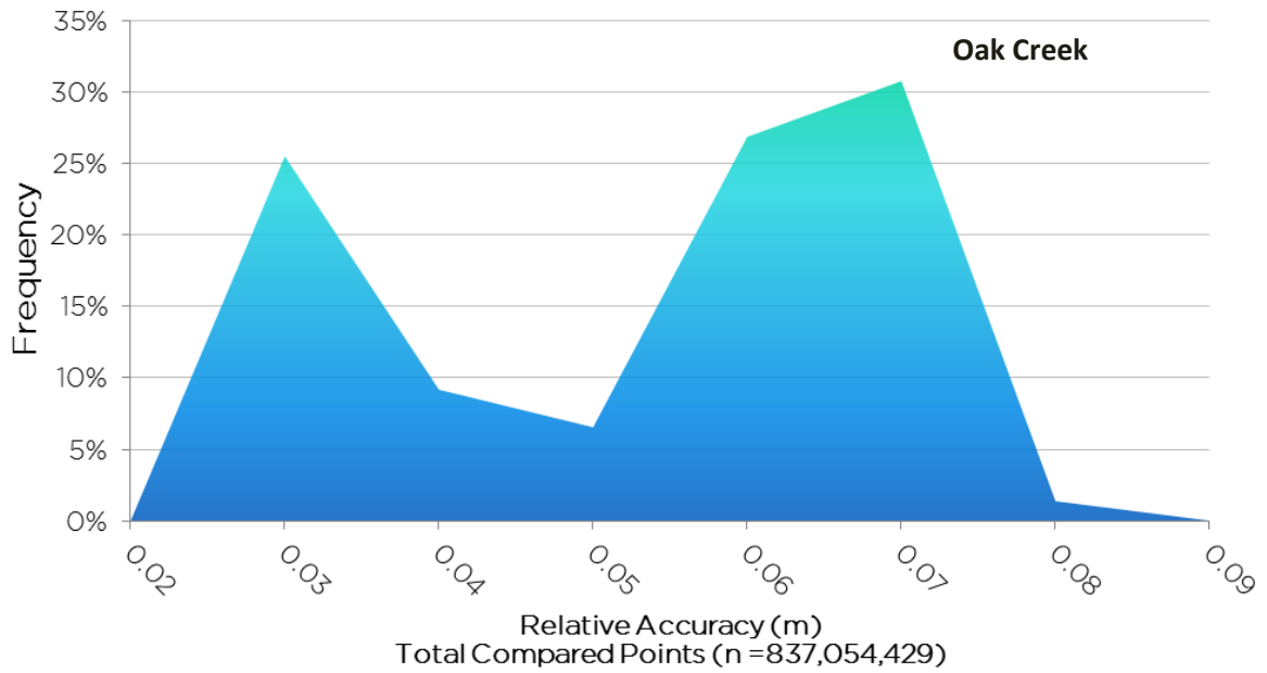
Frequency plot for relative accuracy between flight lines for the Oak Creek AOI
