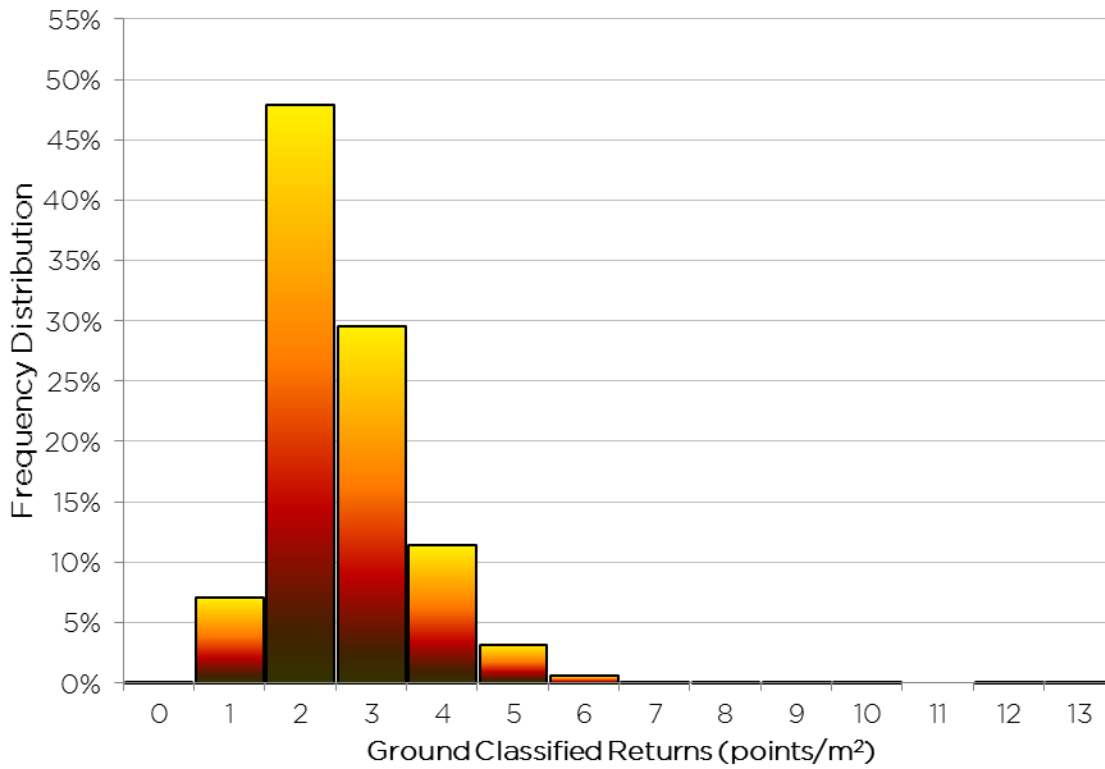
Figure 4: Cumulative frequency distribution of ground return densities of the 1m gridded study area for all 5 delivered AOIs
