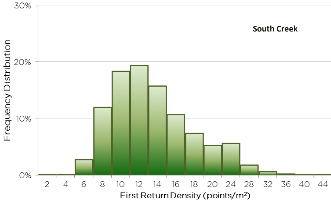
Frequency distribution of first return densities (native densities) of the 1m gridded study area for the South Creek AOI
