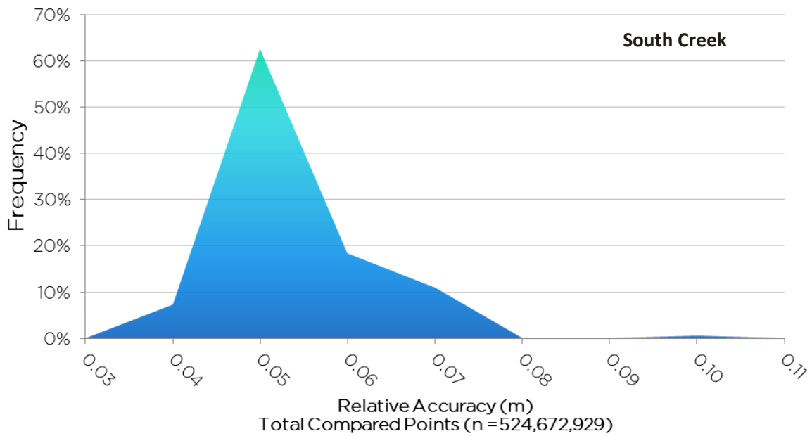
Frequency plot for relative accuracy between flight lines for the South Creek AOI
