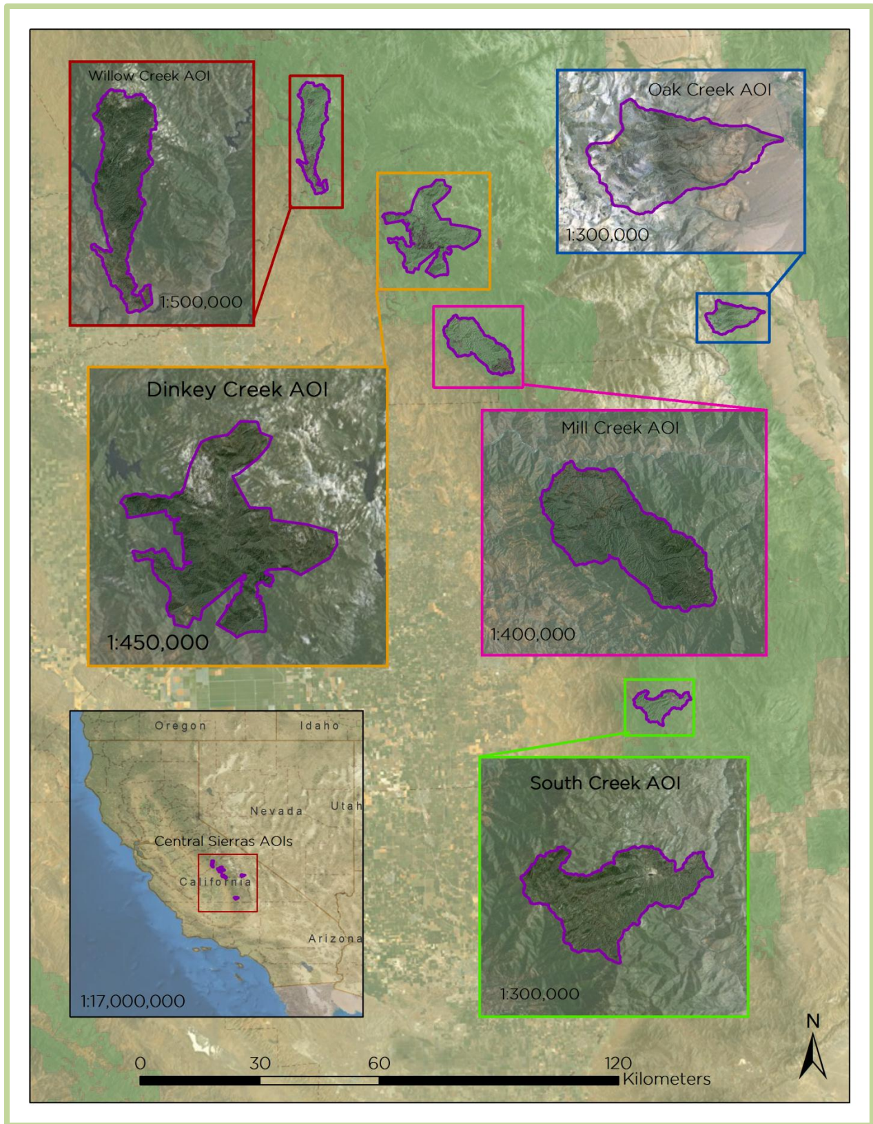
Figure 1: Location map of the delivered USFS Region 5 LiDAR sites in the Central Sierras
