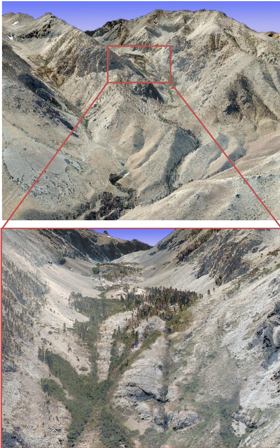
Figure 10: Two views looking west up South Fork Oak Creek at a riparian area below Parker Lakes in the California Bighorn Sheep Zoological Area. Images created from the LiDAR point cloud colored by 2010 NAIP Imagery.
