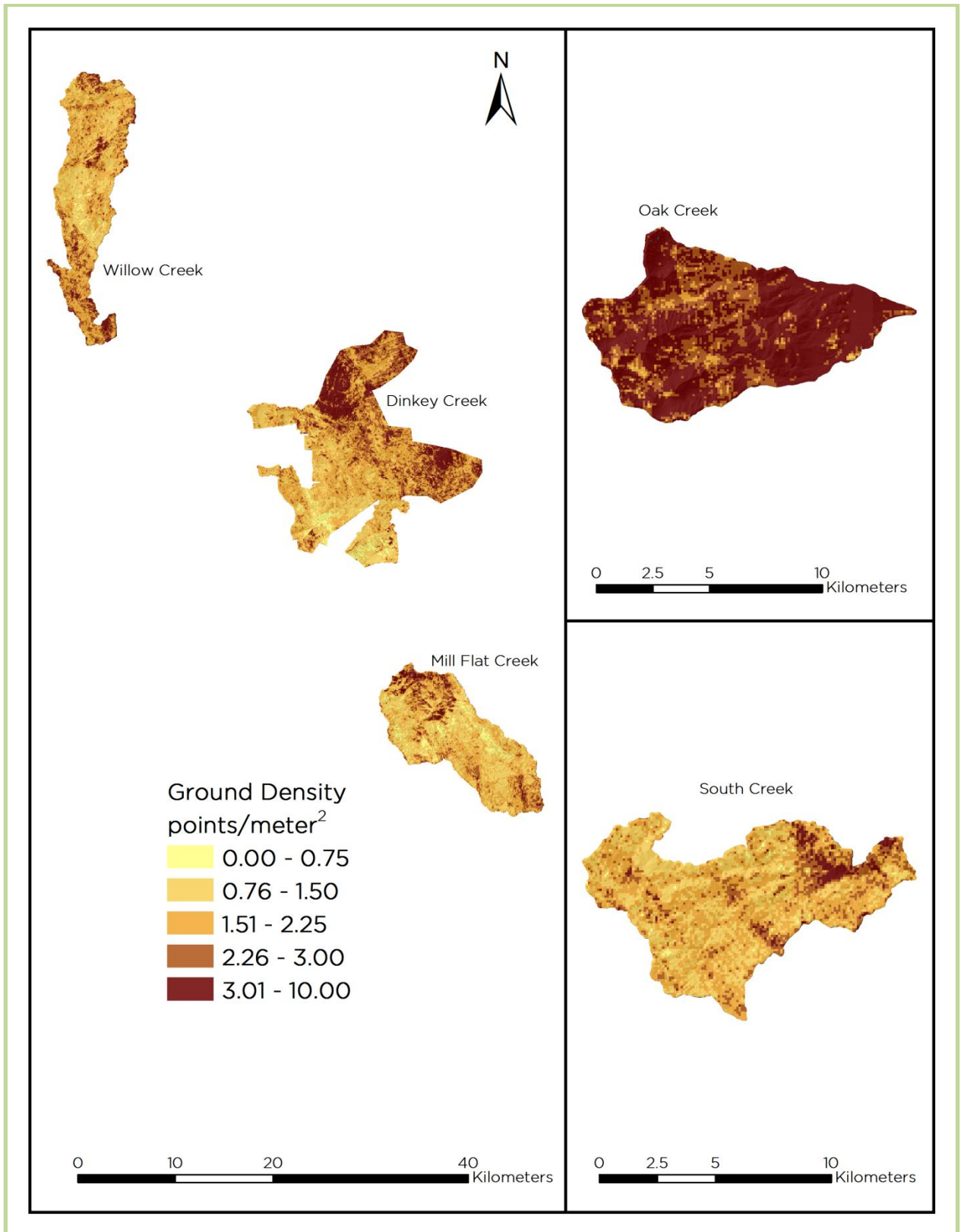
Figure 6: Ground density map for the Central Sierra AOs
